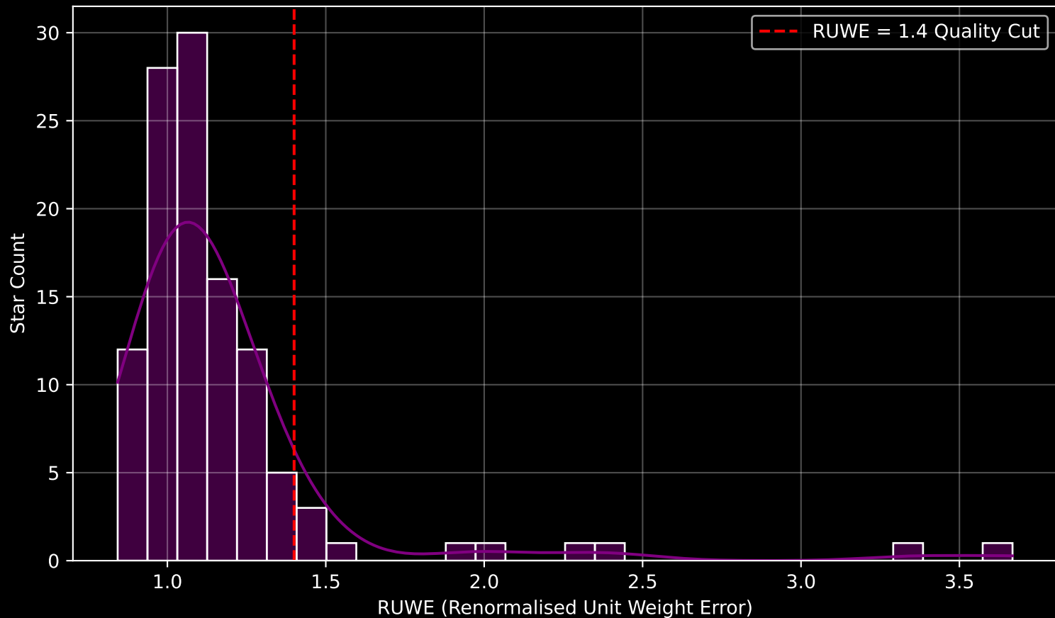
GALAH DR4 Field [6692] RUWE Distribution (n= 113)
