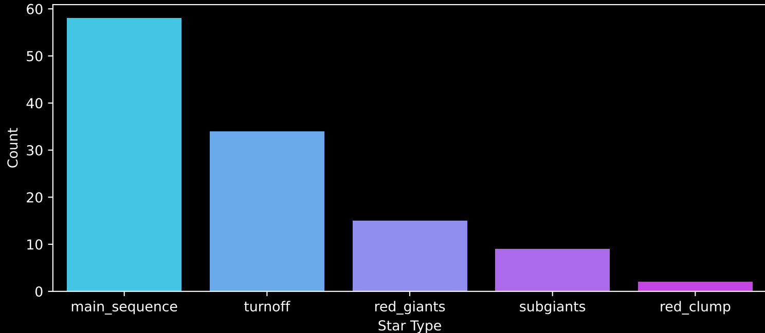
GALAH DR4 Field: [6692] Count plot of Star Type
