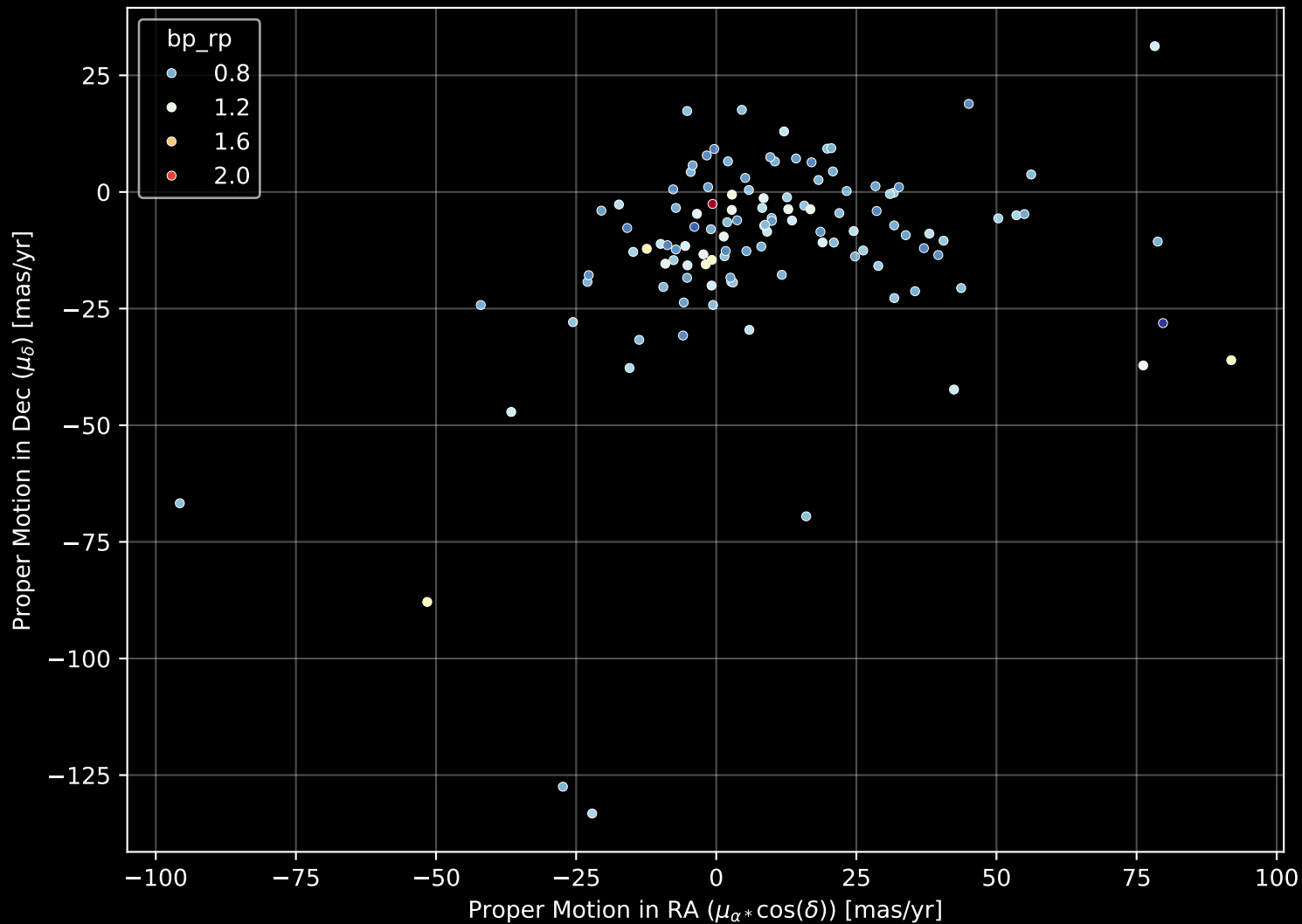
GALAH DR4 Field: [6692] Proper Motion Diagram (n= 118)
